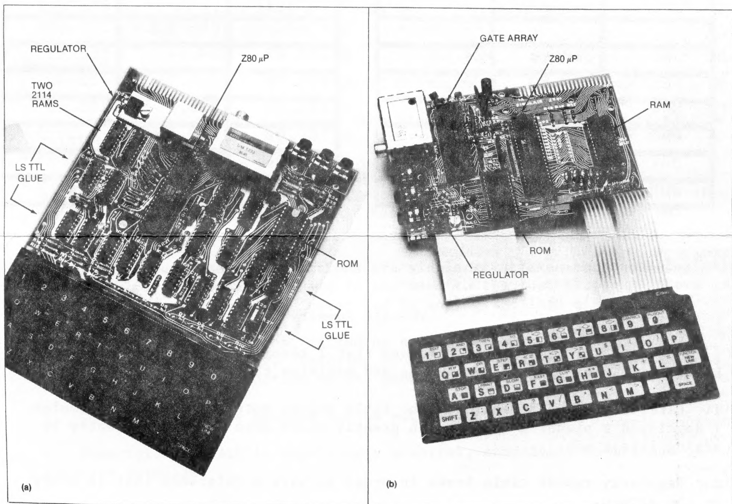
Seventeen LS TTL glue parts (gates, latches, drivers, etc) combine with a Z80 \mu P, a 24-pin ROM and two 2114 RAMs in Sinclair's original design for its ZX80 personal computer (a). The redesigned unit (b) uses only four ICs: the Z80, the 24-pin ROM (in a byte-wide 28-pin socket for future expansion), a 4118 byte-wide RAM and a Ferranti ULA 810 2 gate-array IC.
